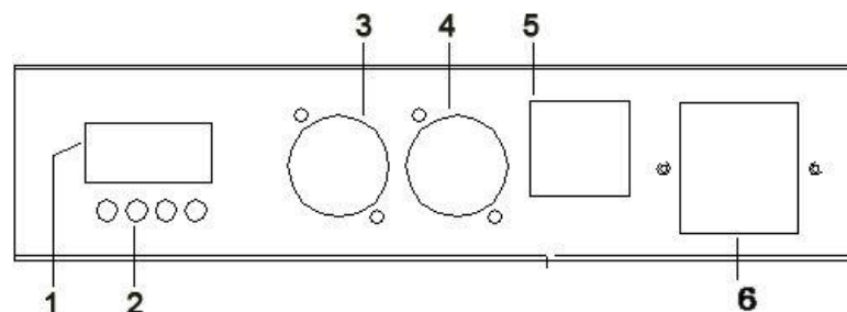
1. Alpha-numeric display 2. Touch switches 3. DMX-Out socket 4. DMX-In socket 5. Power out 6. Power in
