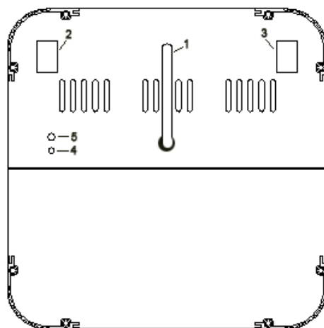
1. Antenna 2. Power switch for wireless receiver 3. Power switch for battery power 4. Wireless indicator 5. ID code selector
